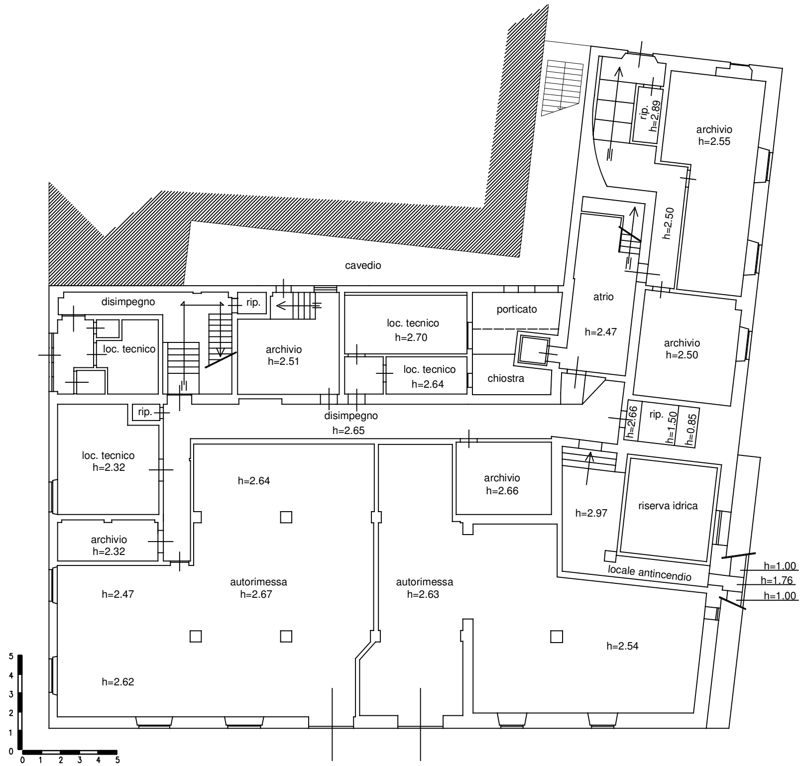
PIANO SEMINTERRATO
