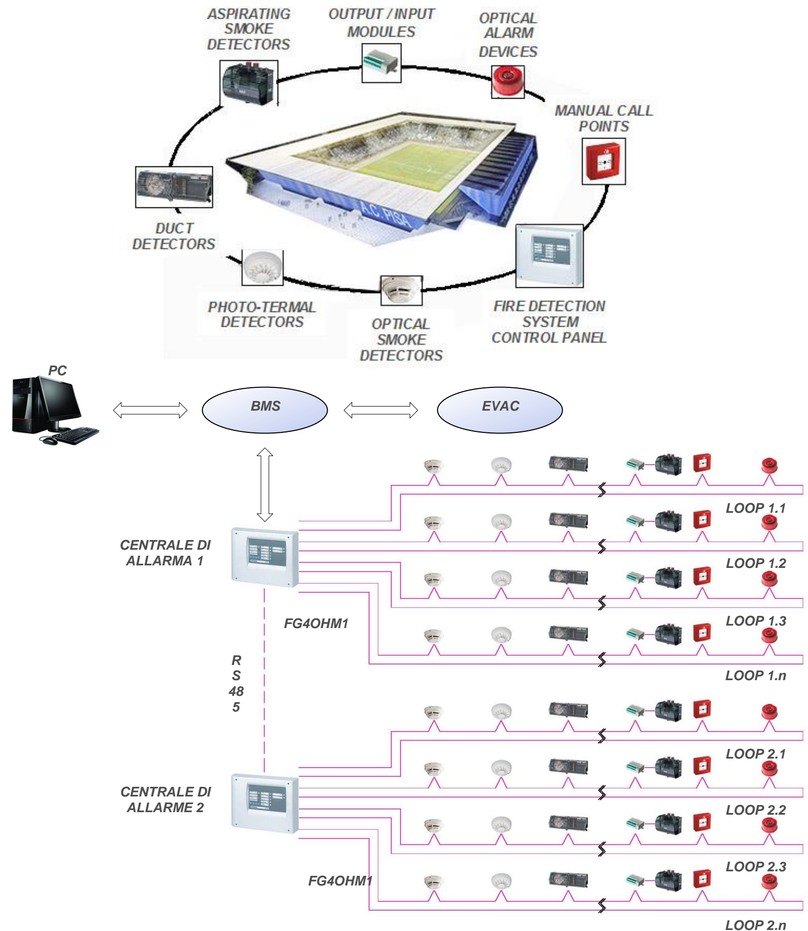
Fire-detection system
